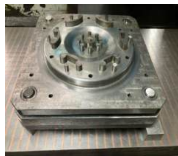
Automobile Industries Compound Die for Flex Plate (Aulternate forFly Wheel)
